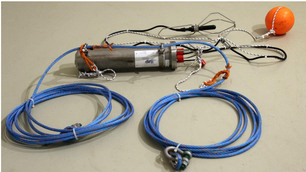
Figure 10: Underwater noise measurement device of the itap GmbH; at the very back, the hydrophone with floatation body.
