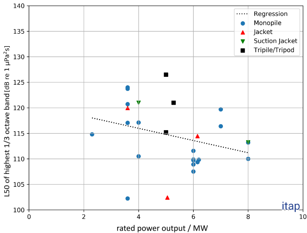
Figure 21: L 50 of the 1/3-octave band with the highest level in 100 m distance from the OWTG as function of their nominal power. Top: independent of foundation structure; below: broken down by foundation type.
