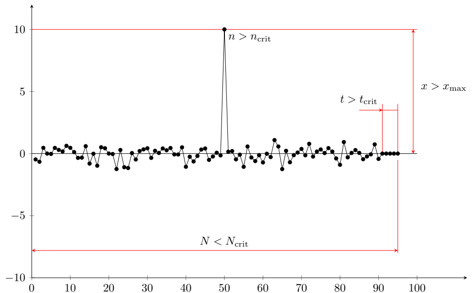
Figure 1 – Artificial time series of length N < N_{\text{crit}} illustrating the thresholds employed in the quality-control procedure of the RAVE data (see also Table 3 ). Other thresholds are the partial flat line length t_{\text{crit}} , the number of spikes n_{\text{crit}} , and the measurement range x_{\text{max}} , where x_{\text{max}} is the maximum allowable value.
